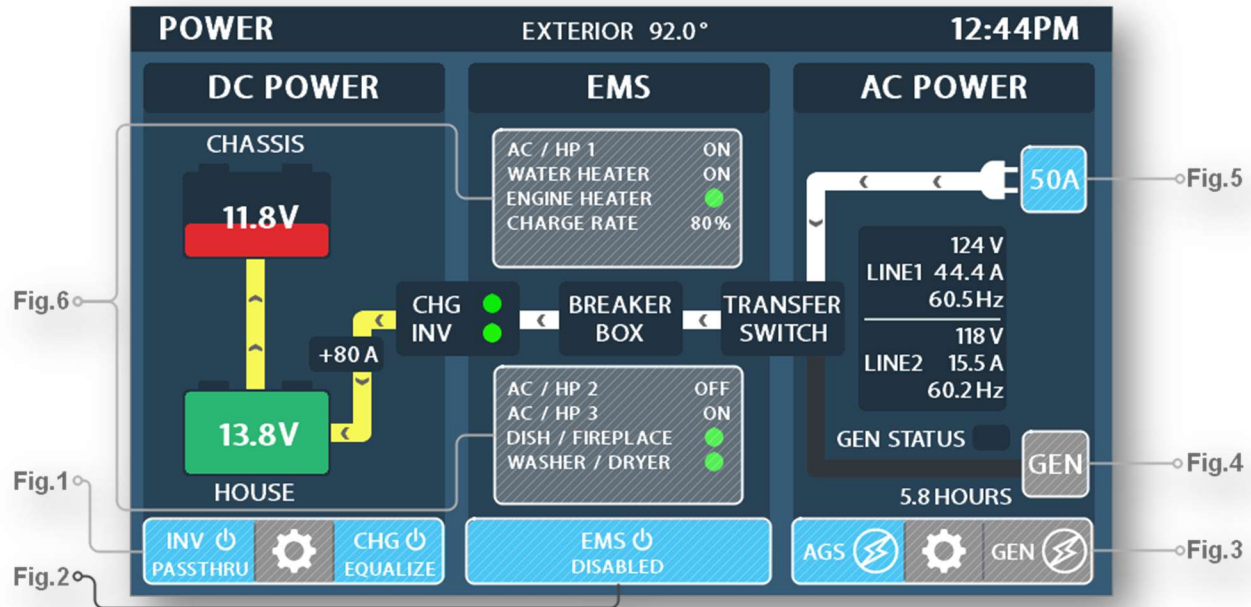
Figure 1 (Inverter / Charger Control + Settings)
