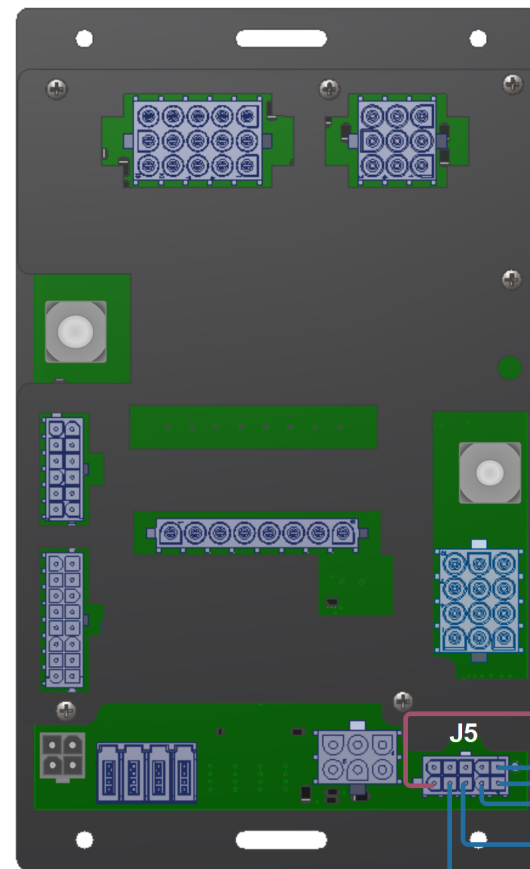
G12 Panel @ Foot of Bed Tiffin P/N: 5104413
