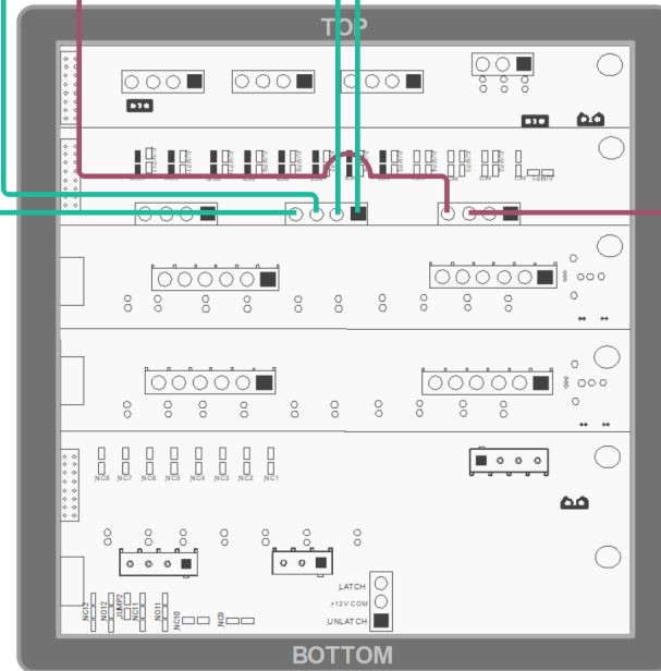
G6 Chassis Panel @ Rear Closet Tiffin P/N: 5083668
